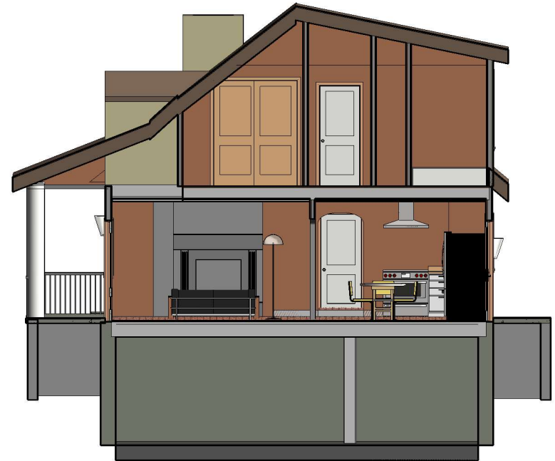
② Side Section 2
